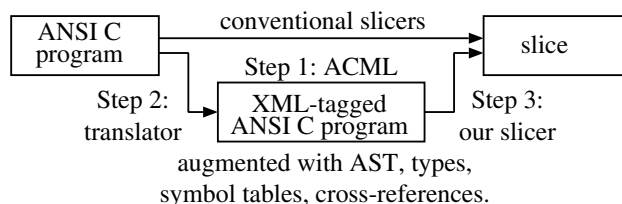
Figure 4. Weiser’s program slicer based on ACML
