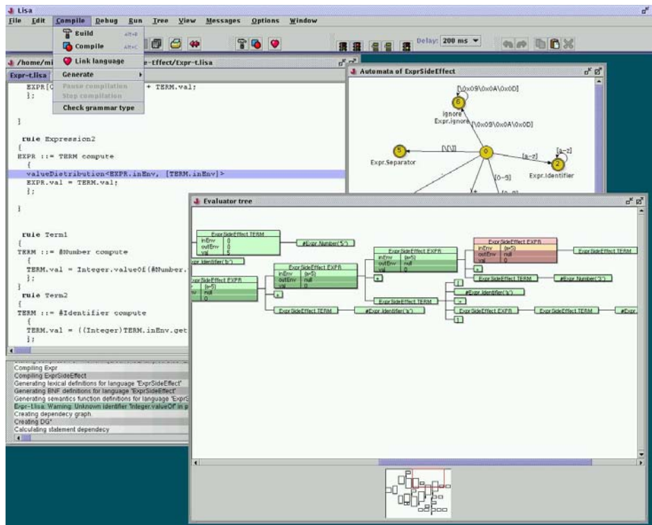
Figure 1: LISA Integrated Development Environment
