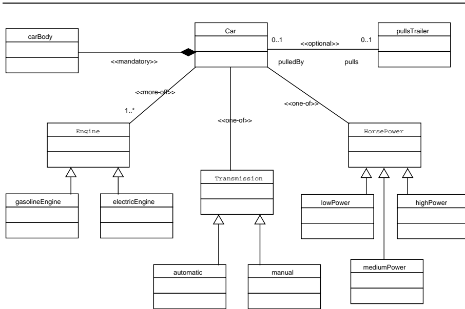
Figure 13: UML Class Diagram for Car Features
