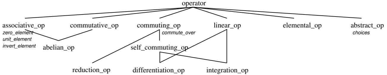
Figure 8: Operator Class Hierarchy
