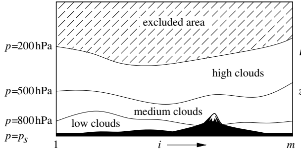
Figure 5: Schematic Illustration of Three Cloud Layers
