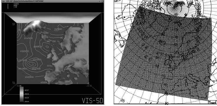
Figure 2: HIRLAM Weather Forecast and Grid Mapping
