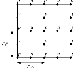
Figure 3: Horizontal Arrangement of Variables on an Arakawa-C Grid
